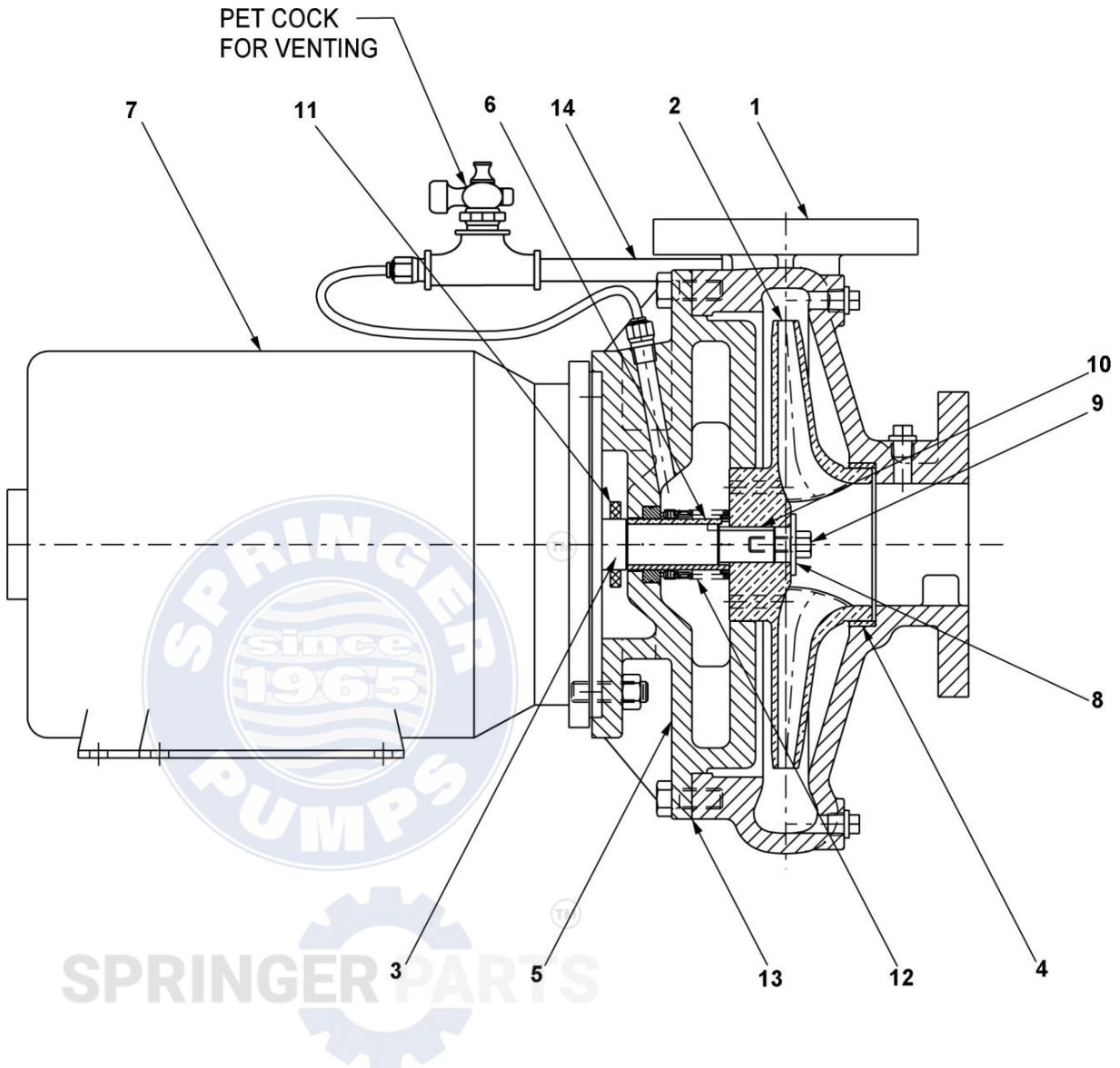
Figure 2 – Repair Parts Illustration
