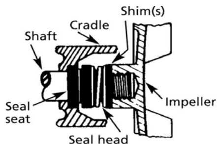
Figure 1 – Mechanical Seal Replacement
