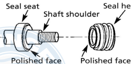
Figure 1 – Mechanical Seal Replacement
